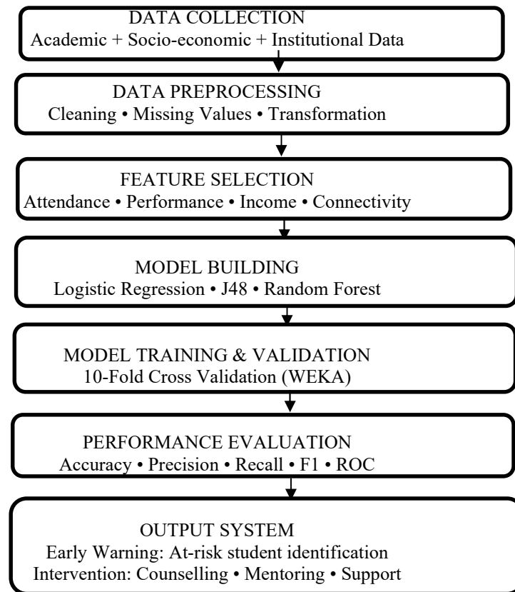
Fig.2 Proposed Machine Learning Model.
